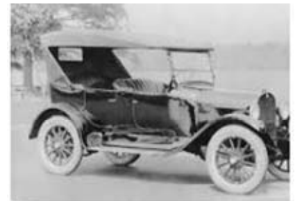
1922 DODGE TOURING CAR
